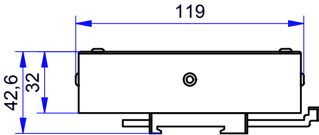
DIN-holder HS35
