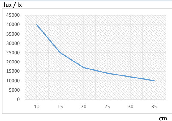
Messung der Helligkeitsabnahme in Abstand in cm / measuring of the reduction of brightness in cm distance
